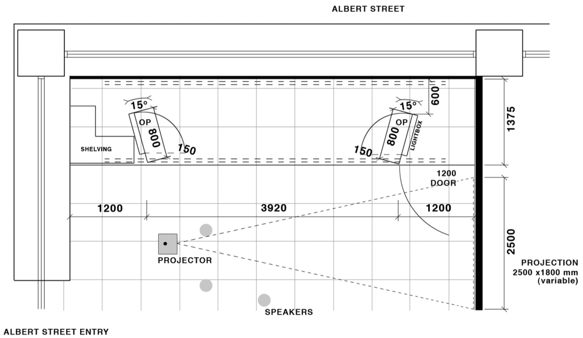
FLOOR PLANS
