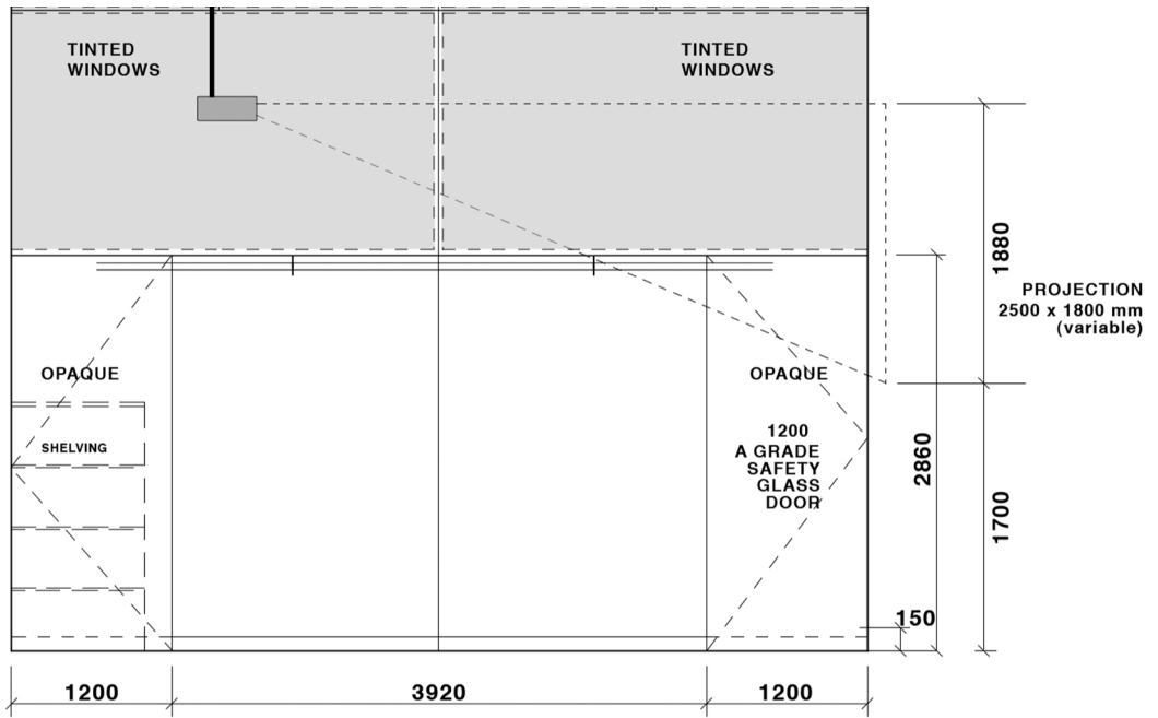
SIDE ELEVATION
